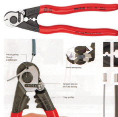
KPX9561190 Wire Rope Cutter 7mm Knipex • Two crimping dies for end caps on Bowden cable sheaths and end ferrules for traction cables. • Cutting-edge hardness approx. 64 HRC • Chrome vanadium heavy-duty steel, forged, oil-hardened.
